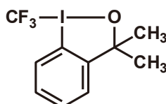
Togni Reagent
