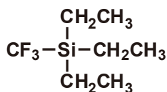
Triethyl(trifluoromethyl)silane
