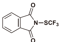
N-(Trifluoromethylthio)phthalimide
