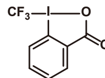
Togni Reagent II
