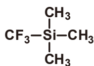
(Trifluoromethyl)trimethylsilane (Ruppert-Prakash Reagent)
