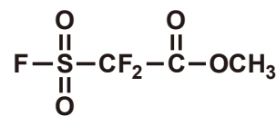
Methyl Fluorosulfonyl- difluoroacetate
