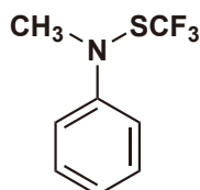
N-Methyl-N-(trifluoromethylthio)aniline 200mg / 1g
