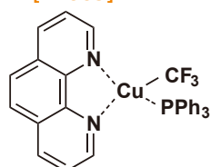
(1,10-Phenanthroline)-(trifluoromethyl)-(triphenylphosphine)copper(I)
