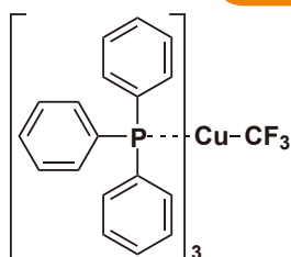
(Trifluoromethyl)-tris(triphenylphosphine)copper(I)
