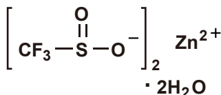
Zinc(II) Bis(trifluoromethanesulfinate) Dihydrate
